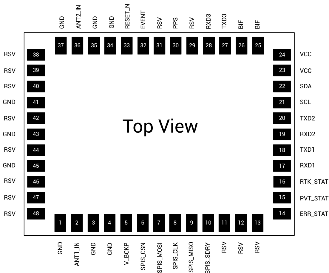
Figure 2-1 UM982 Pins
