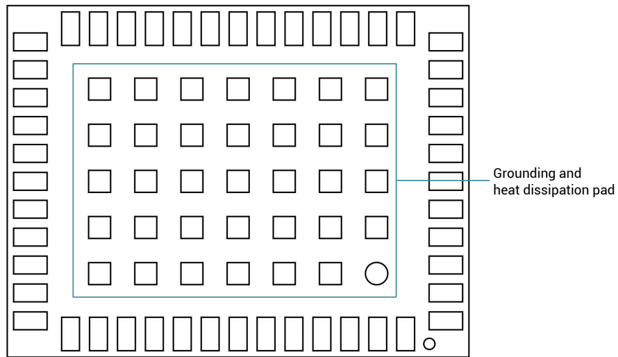
Figure 3-3 UM982 Grounding and Heat Dissipation Pad (Bottom View)
