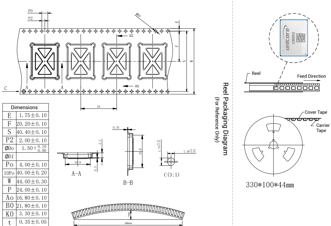
Figure 5-3 UM982 Reel Package Diagram
